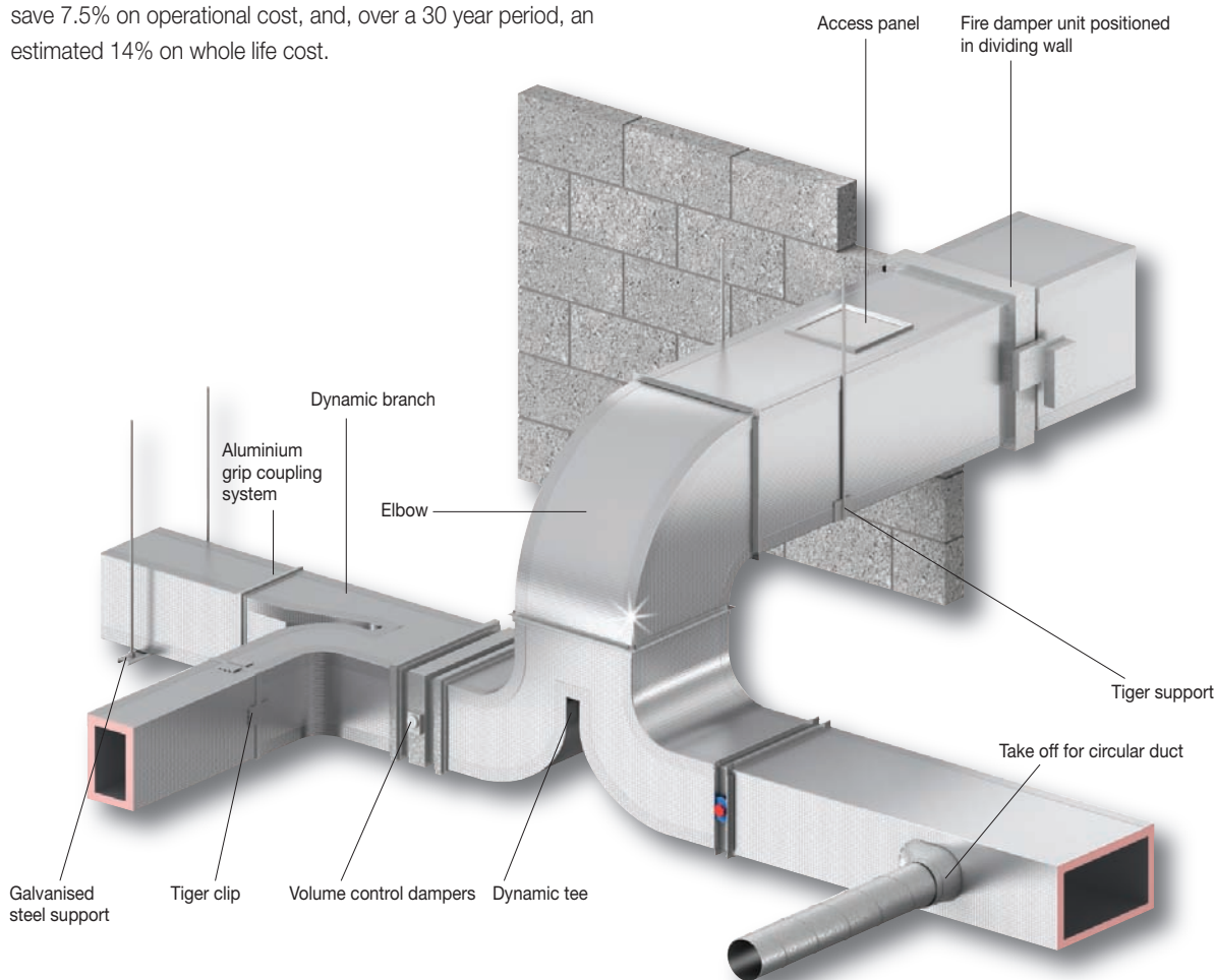
Figure 1: The Kingspan KoolDuct® System of Pre-insulated Ductwork
